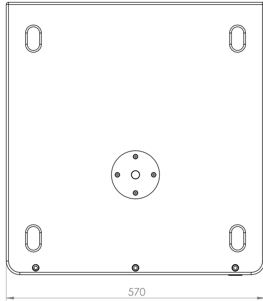
Top View
